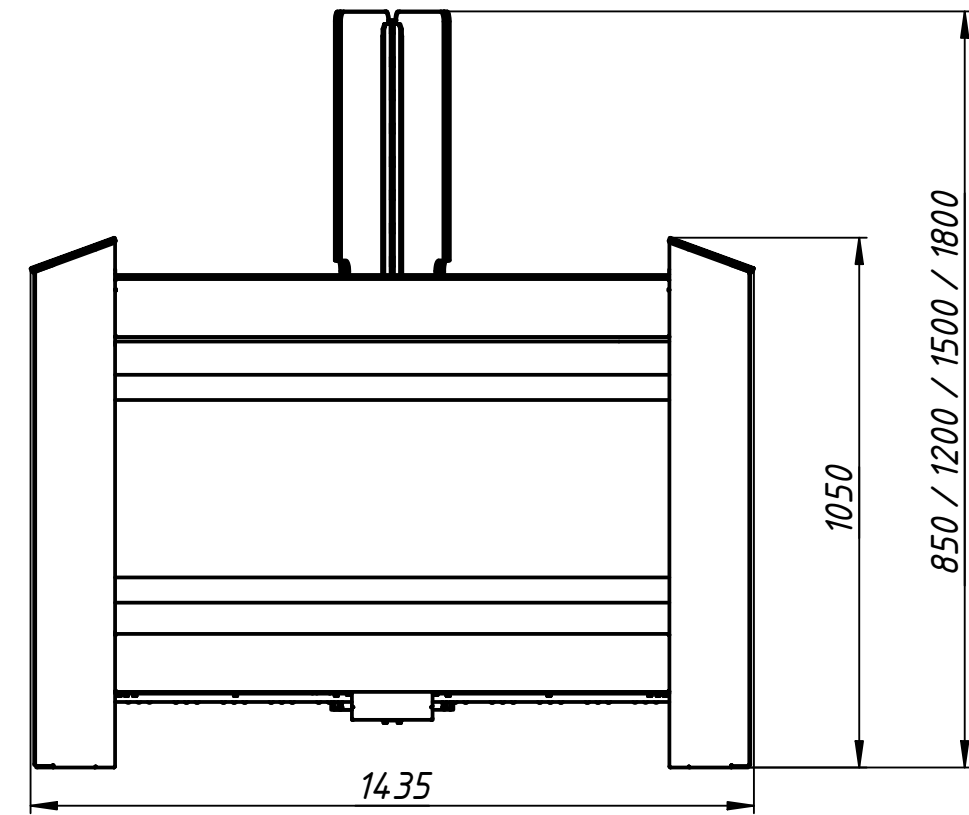
Installation template
