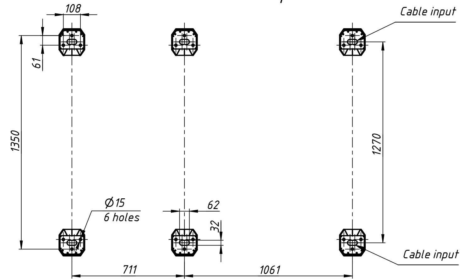
Installation template
