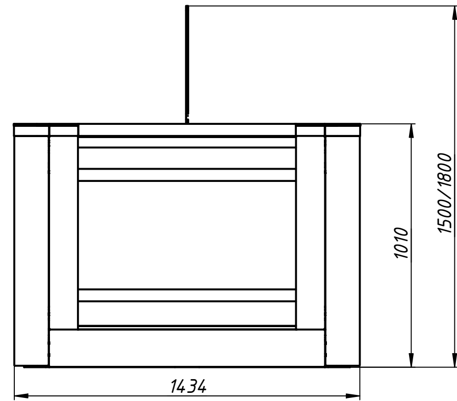
Installation tamplate
