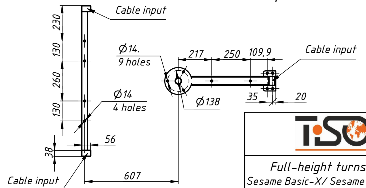
Installation tamplate
