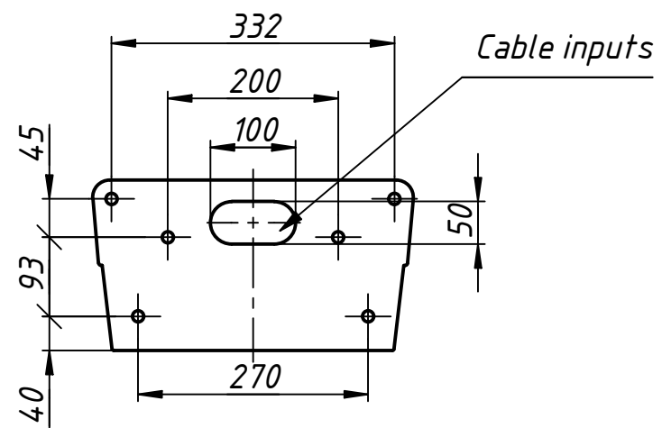
Installation tamplate
