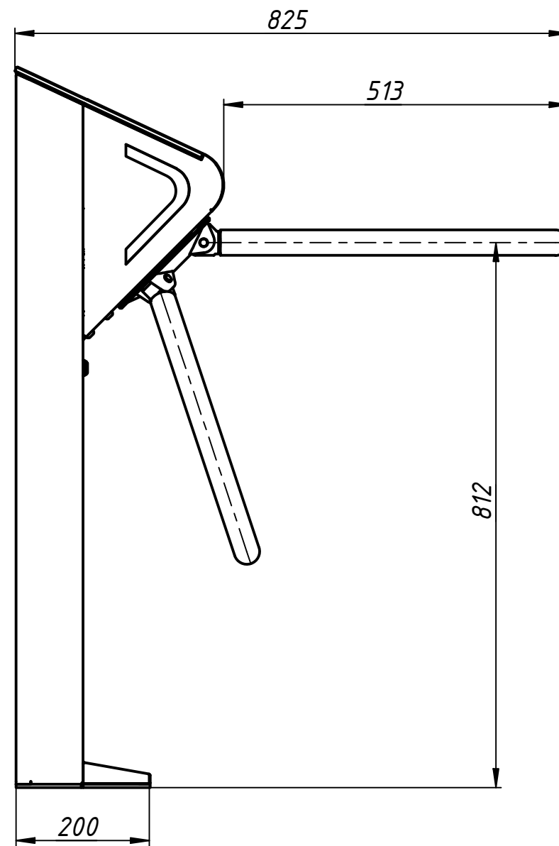
Installation tamplate
